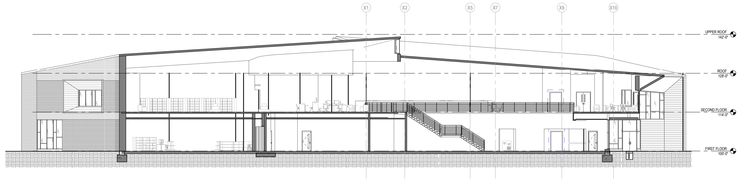
1 EAST-WEST 3/64" = 1'-0"
