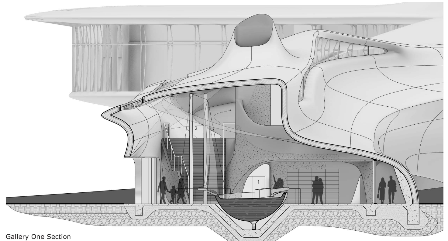
Gallery One Section (S5) Scale(~) 3/32" = 1'
