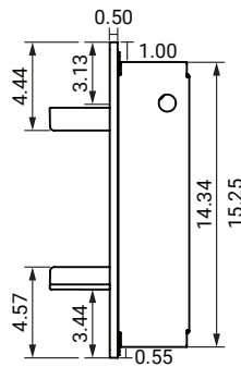
ATTACHMENT OPTION B HOLES FOR ATTACHMENT STUDS. USE PAN HEAD SCREWS
